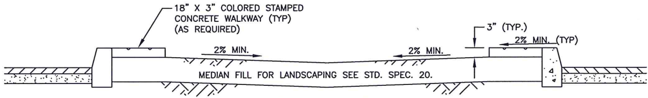
MEDIAN DETAIL
